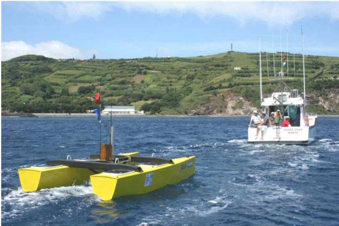
The Catamaran DelfimX (ISR/IST, Portugal) and the Research Vessel Águas Vivas (IMAR, Portugal) performing an automatic “follow the leader” maneuver in the area of the Azores.
